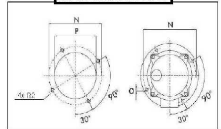
FRT-R1-50/51/60/64/66 FR1-50 / 51 / 52 / 60 / 61 / 64
