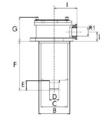
FRT-R1-10/20/22/30 FR1-10 / 20 / 21 / 22 / 23
