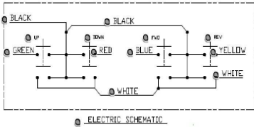
ELECTRIC SCHEMATIC
