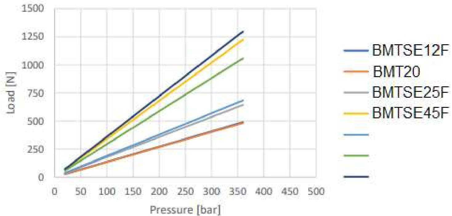
Load effort for 550 mm handle
